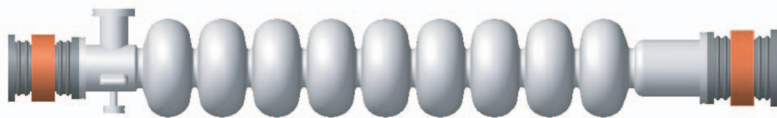
Figure 1: Conceptual view of the KEK-ERL model-2 cavity.
