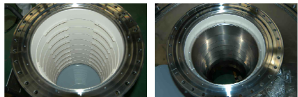
Figure 1: Segmented ceramic insulator, without (left) and with (right) guard-ring electrodes.
