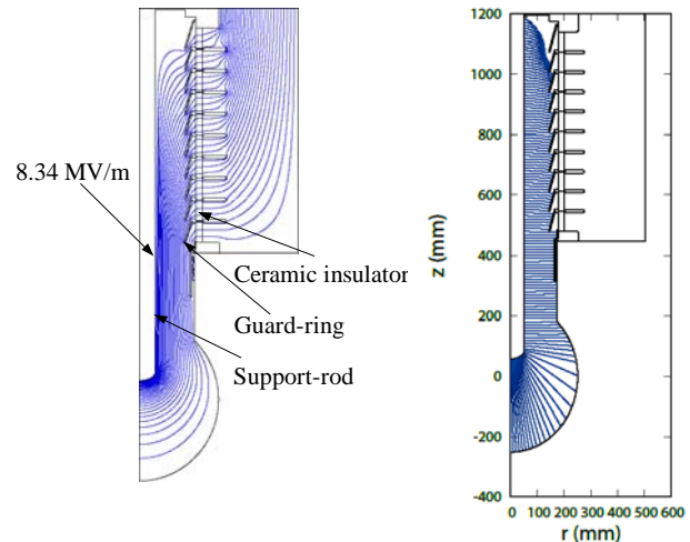
Figure 2: Field distribution (left) and emitted electron trajectories (right) of the gun.
