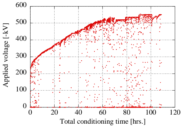
Figure 3: Applied voltage vs total time in the high-voltage conditioning.
