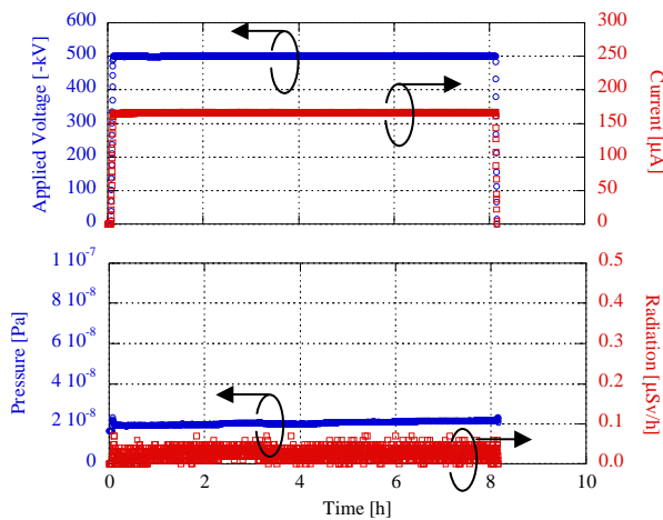
Figure 4: Results of a long-time holding test for 8 h at a generator voltage of 510 kV.
