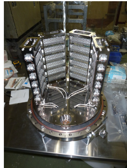
NEG pump set
