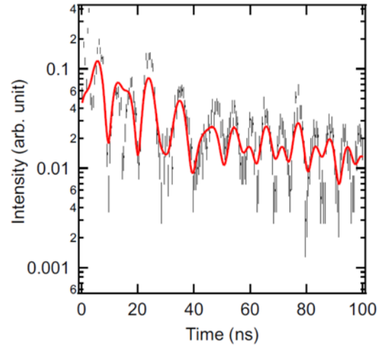
FIG. 4: Experimental data and the fitting curve of the NRS time spectra after cleaning procedure ( Ar^+ sputtering, annealing and O_2 annealing).
