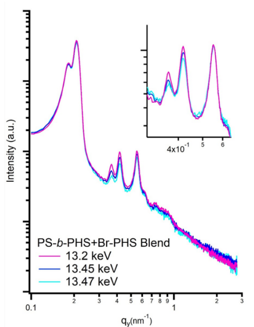
Figure.1 Energy dependence of in-plane GISAXS line profiles.
