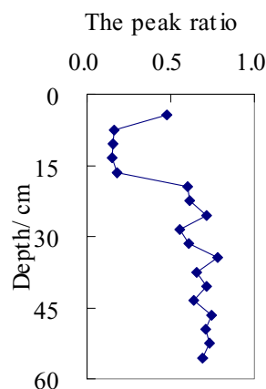
Fig. 2. The vertical distribution of the peak ratio of the two sharp peaks in sulfur XANES spectra of the Yatsu tideland sediments
