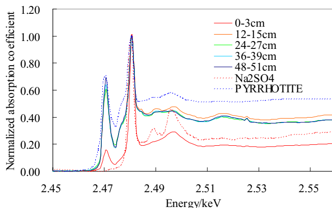
Fig. 1. Normalized sulfur XANES spectra of the Yatsu tideland sediments and standard materials
