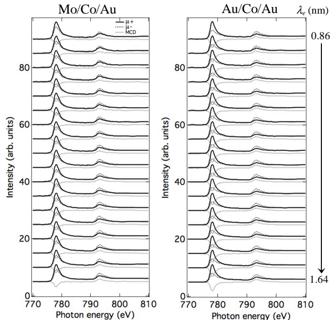
Figure 1: Co L -edge XAS and XMCD spectra for the Mo/Co/Au and Au/Co/Au films for different probing depth at normal incidence. These spectra are taken at the position of the sample where the Co thickness \sim 0.9 nm where perpendicular magnetic anisotropy was observed in the both samples. The probing depth, \lambda_e , was varied in the range from 0.86 nm to 1.64 nm.
