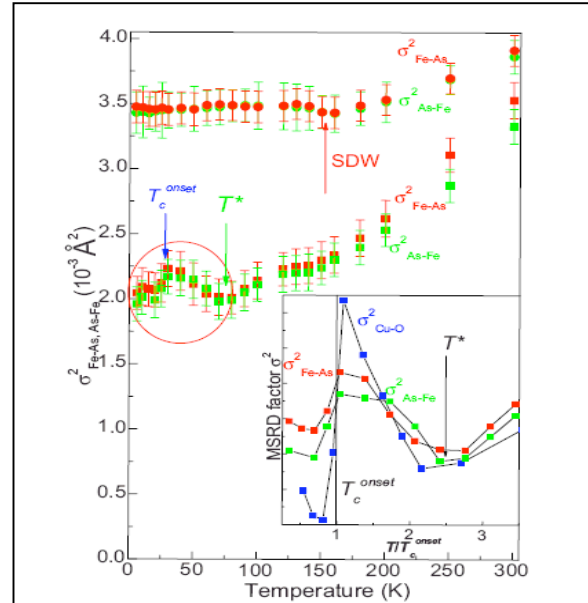
Fig. 1 Temperature dependence of Fe-As bond mean-square relative displacements for \text{LaFeAsO}_{0.93}\text{F}_{0.07} (squares) and \text{LaFeAsO} (circles). The red symbols are derived from Fe K edge EXAFS measurements and the green symbols are derived from As K edge EXAFS measurements. The inset shows an enlarged view of low temperature ( T < 100 K) mean-square relative displacements (MSRD) for the \text{LaFeAsO}_{0.93}\text{F}_{0.07} sample plotted as the function of normalized temperature ( T/T_c^{\text{onset}} ) and the comparison with \text{La}_{1.85}\text{Sr}_{0.15}\text{CuO}_4 .
