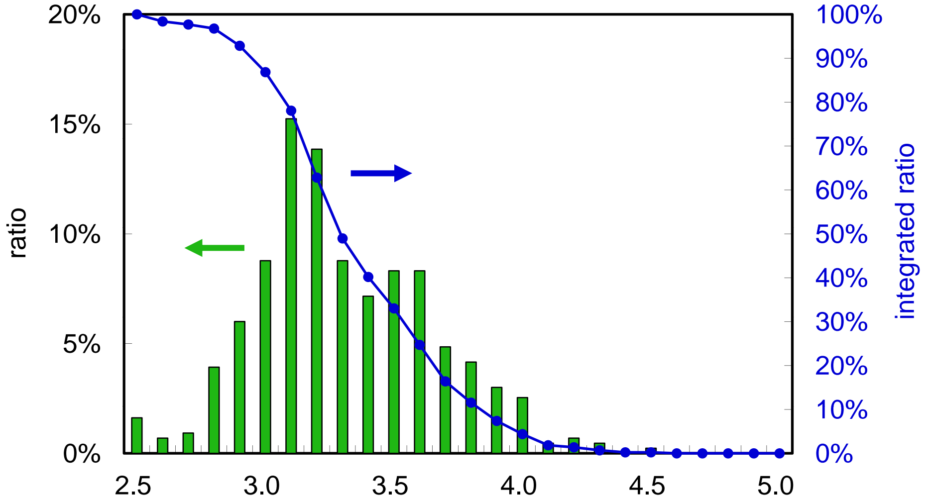
Distribution of approved proposal scores in FY2011 (Category G)
